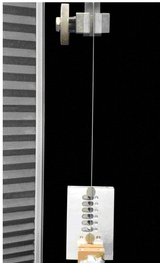
Figure 4 - Device positioned in the Instron machine.
