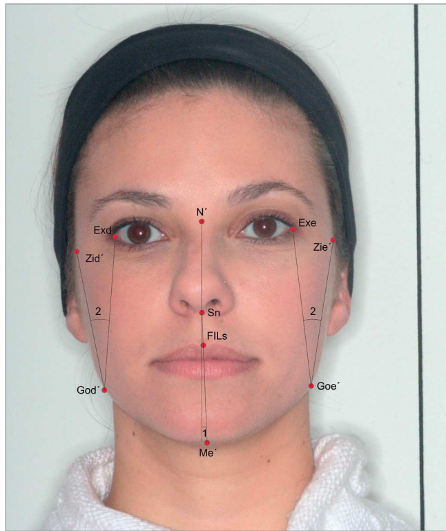
Figure 6 - Angular measures 1 and 2: 1) Facial symmetry angle - angle formed between facial midline (N'-F) and Sn'Me' line 2) Symmetry between left and right side of the face - the difference between left and right angle measurements formed by intersection of Zi'-Go' and Ex-Go' lines
