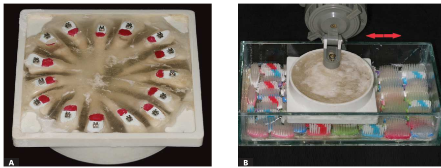
Figure 9 - A) Teeth attached to a sink strainer so as to form a single specimen to be taken to the brushing machine; B) Brushing machine comprised by a glass box with tooth brush heads attached to the bottom with hot glue. The engine of a security camera was adapted to perform round-tripping movements.
