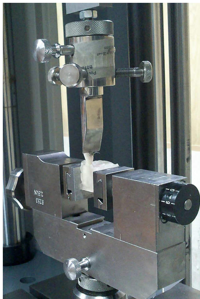
Figure 1 - A 0.6-mm metal blade was used to apply shear force to the composite interface.
