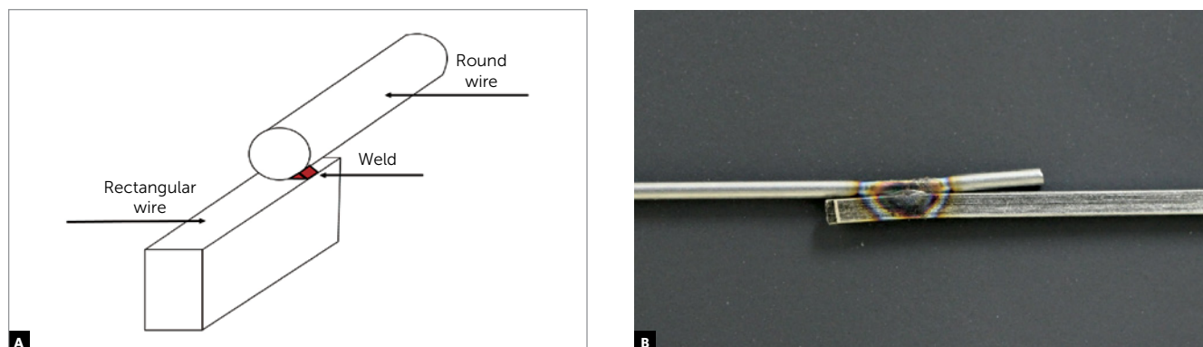
Figure 1 - A) Schematic drawings of the electric resistance weld. B) Image of a weld analyzed in this study.
