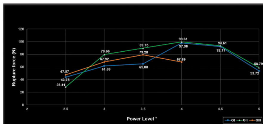
Figure 2 - Graph of maximum tensile strength of the welds performed in NiTi wires of the tested groups, according to the used power levels. * One unit of power level of the welding machine represents 500W.
